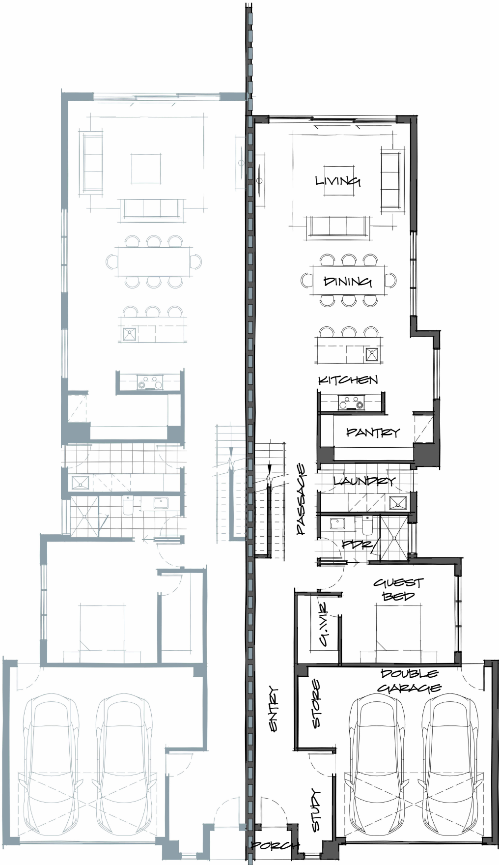
Ground Floor
