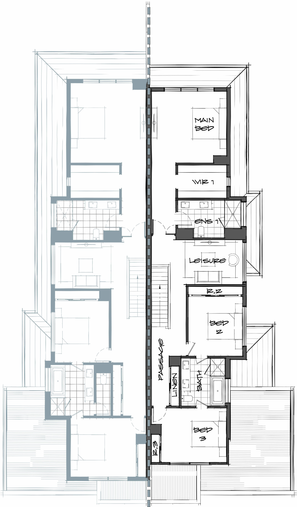
First Floor
